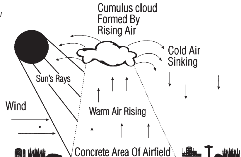
Fig 4-7 Thermal Conditions
