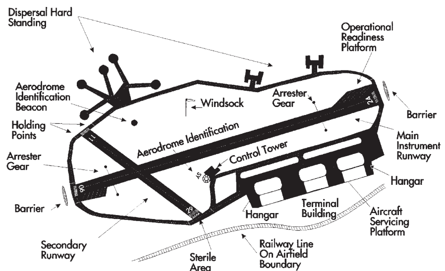
Fig 1-1 Typical layout of a main instrument runway
