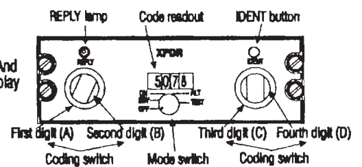
Fig 5-5 SSR Set
