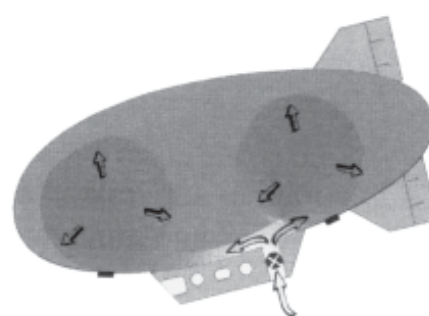
Fig 1-7 Pumps force air into the ballonets and the airship descends.
